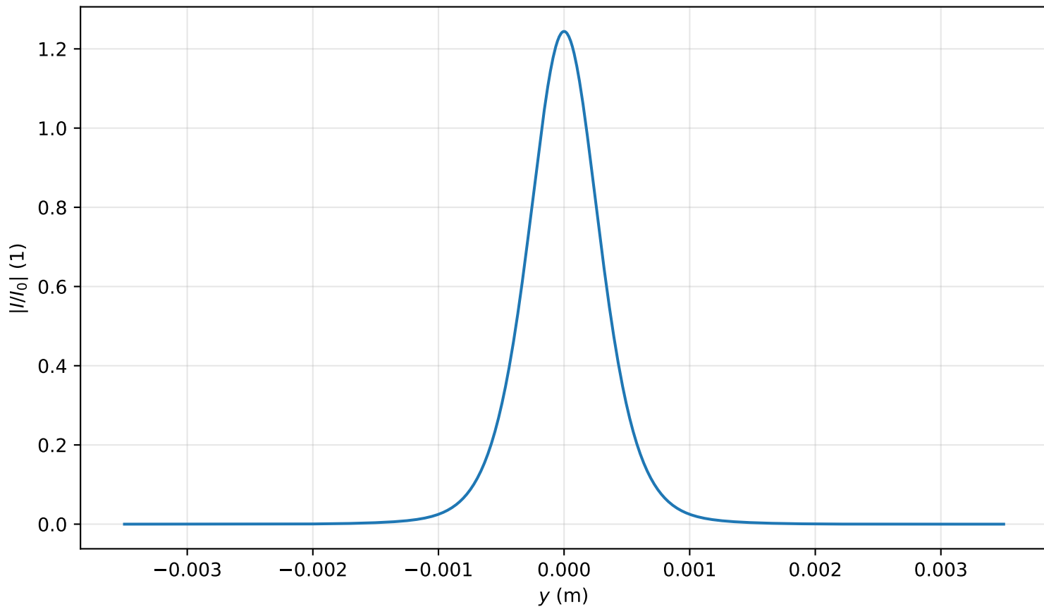
Intensity profile I(x = 0, y, z = 2.388)/I_0 , P_{in}=0.8P_{cr} , artificial time
